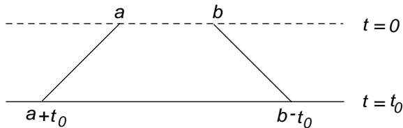
Figure 1: The set \Omega(a, b, t_0) .
